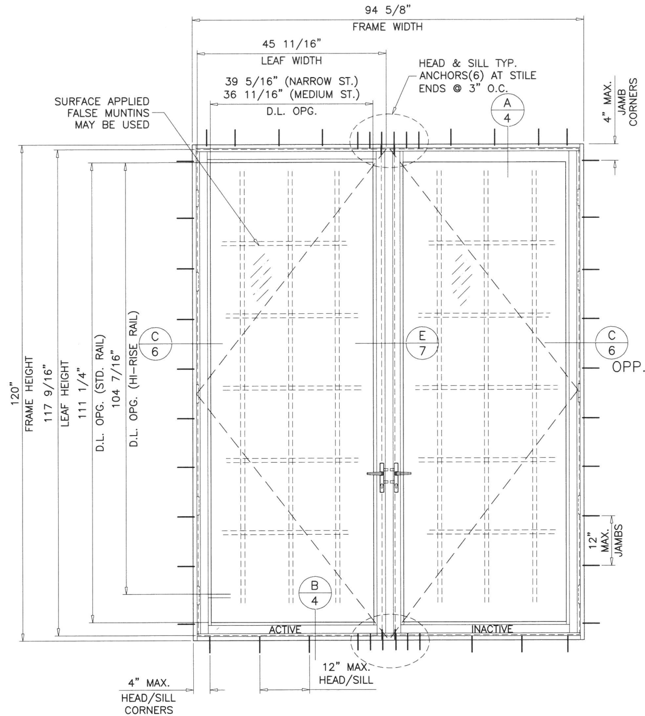
TYPICAL ELEVATION ( XX ) STD. SILL
