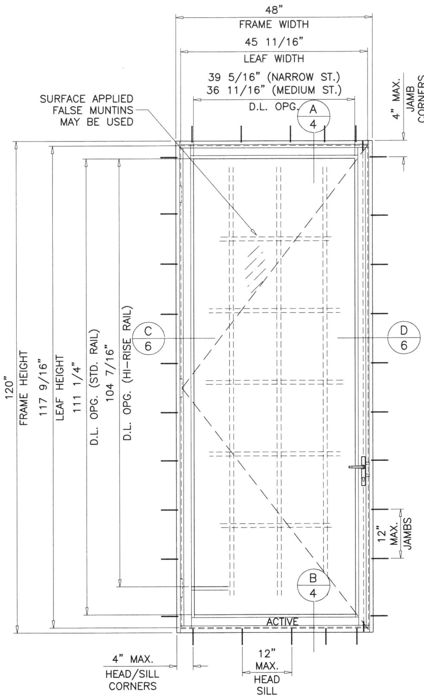
TYPICAL ELEVATION ( X ) STD. SILL
