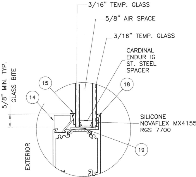
GLAZING DETAIL 1" OVERALL INSUL. GLASS
