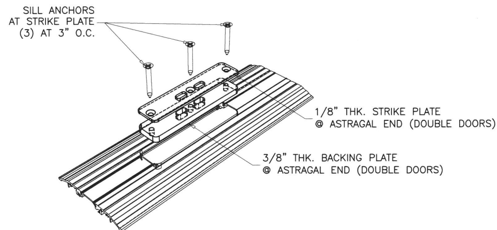
STRIKE PLATES COMMERCIAL SILL DETAIL
